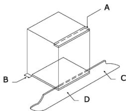
Fig. 8: Ventilation and gap requirements for the installation of a simple electric oven in an upper cupboard.
